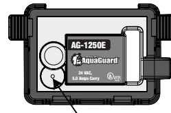
Moisture detection LED
