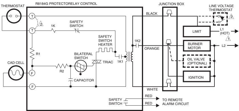
Fig. 1—Typical hookup for TRADELINE R8184G4082 and R8184G4090.
