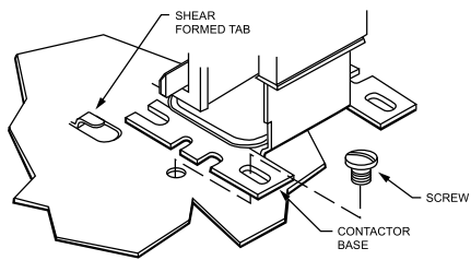
Fig. 1. Typical contactor mounting.
