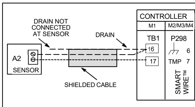
Figure 1. Sensor Wiring
